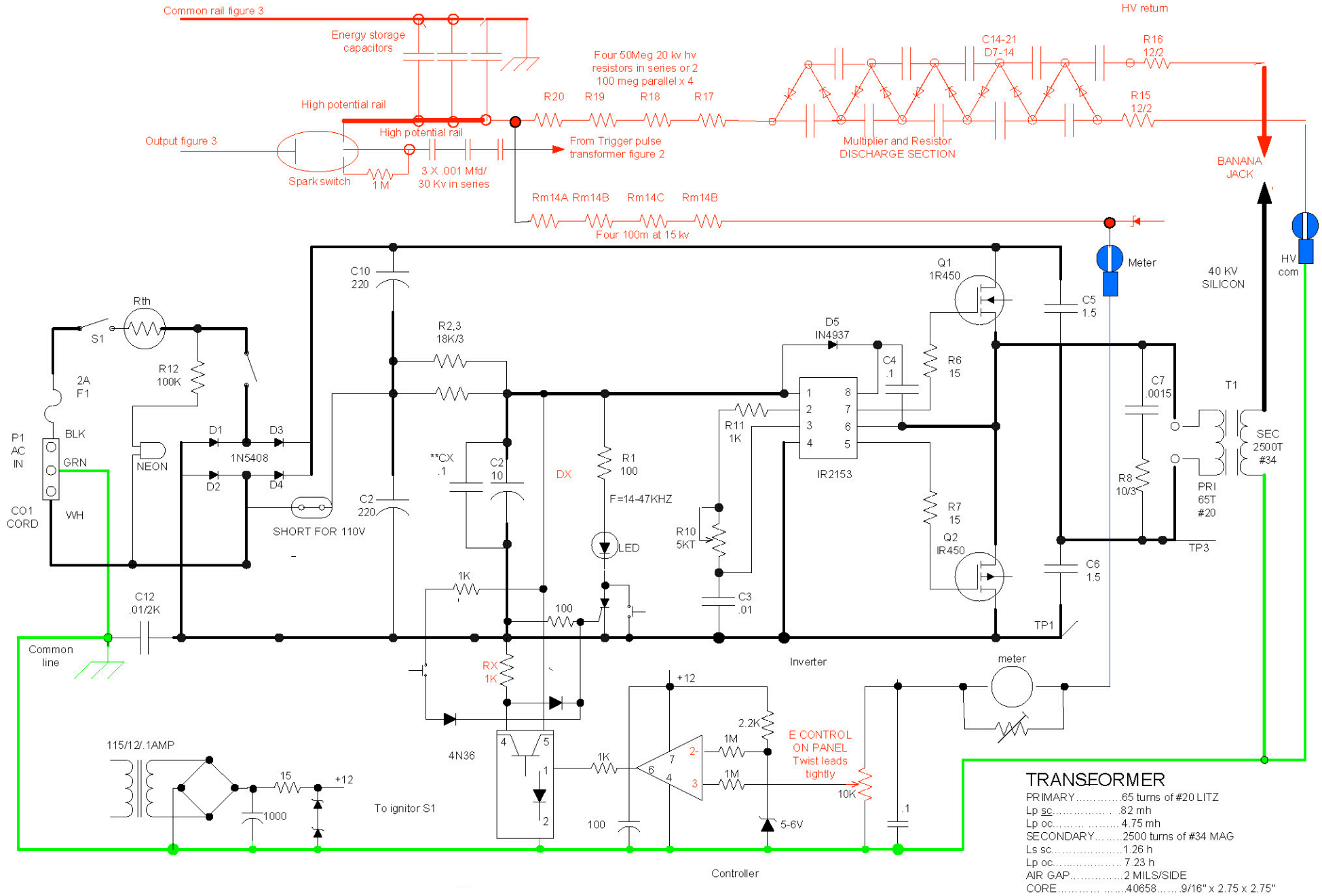
Figure 1 EMP400IU Series Programmable charger and Ignitor
